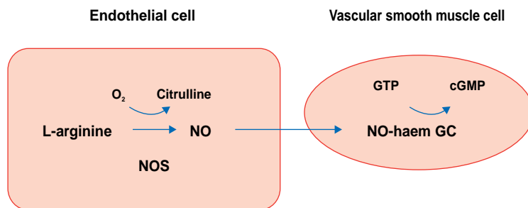
Figure 1. The L-arginine: nitric oxide pathway. NO, nitric oxide; NOS, nitric oxide synthase; GC, guanylate cyclase; cGMP, cyclic guanosine-3',5-monophosphate; GTP, guanosine triphosphate
